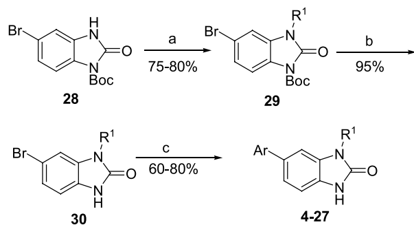
Scheme 1. 6-Aryl-1,3-dihydro-benzimidazol-2-ones. Reagents and conditions: (a) R^1OH , DEAD, Ph_3P , THF, rt or Cu(OAc)_2 , ArB(OH)_2 , CH_2Cl_2 , rt, N_2 ; (b) CH_2Cl_2 , TFA, rt; (c) ArB(OH)_2 , Pd(Ph_3P)_4 , K_2CO_3 , toluene, EtOH/H_2O , 90 °C.
